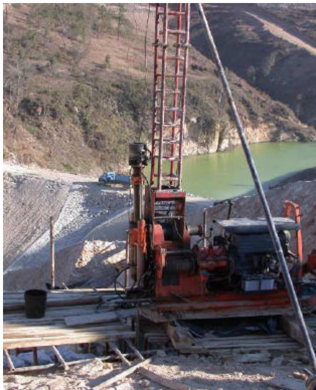
Photo C-6: February 21/22, 2004, Grouting Drill Rig on Left Abutment
